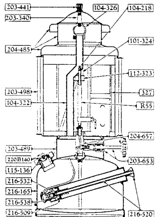
No. L427, Quick-Lite Lantern
